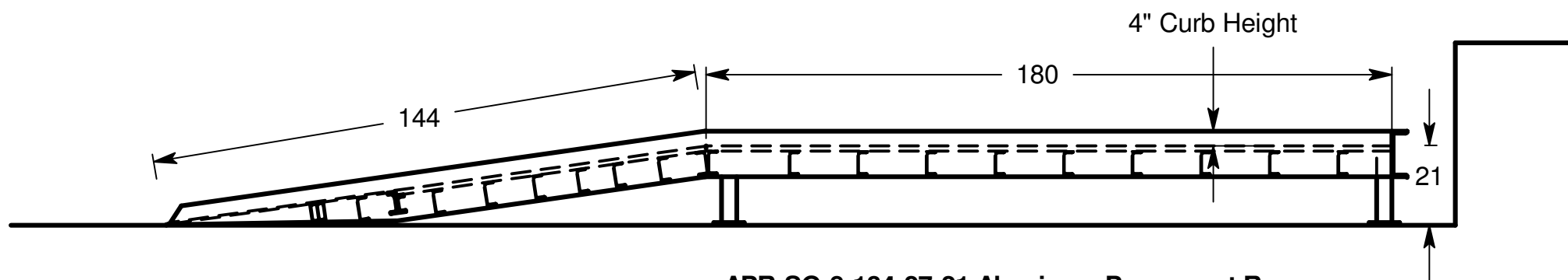
APR-SG-8-134-27-21 Aluminum Permanent Ramp With Serrated Steel Grating 134" overall width - 126" useable 27' long - 12' approach with 15' level off 21" high Weight 4600 lbs.
