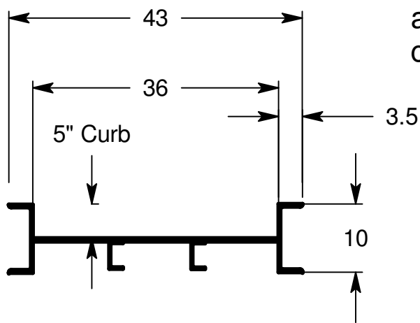
Cross Section
